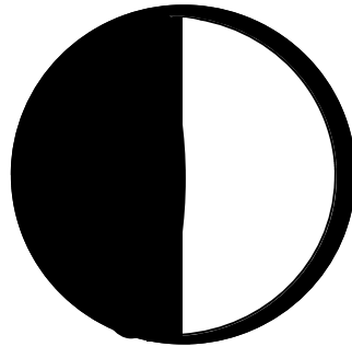
Waxing Half (First Quarter)
