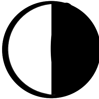
Waning Half (Last Quarter)
