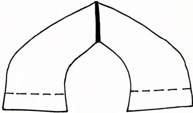
Teapot spout template
